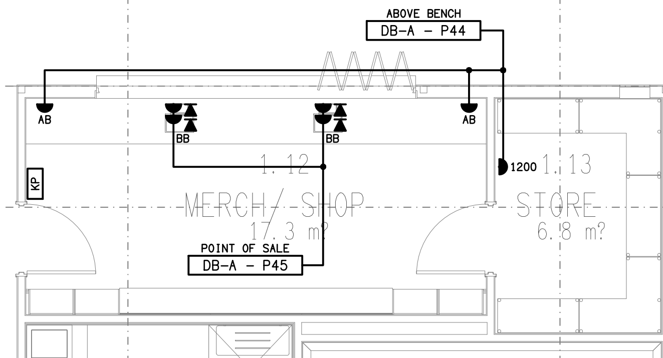
DETAIL B MERCH SHOP FLOOR PLAN
