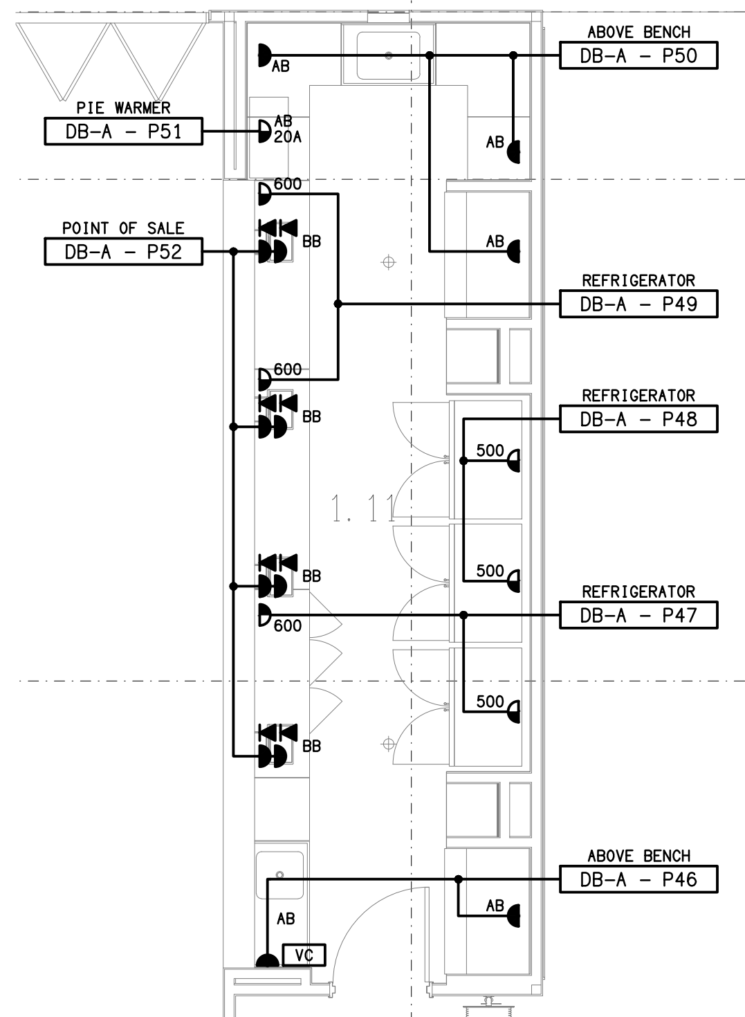
DETAIL C CLUB ROOM BAR FLOOR PLAN
